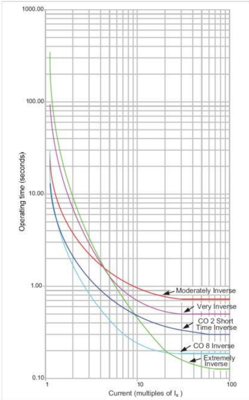
North American IDMT relay characteristics; TD=7
